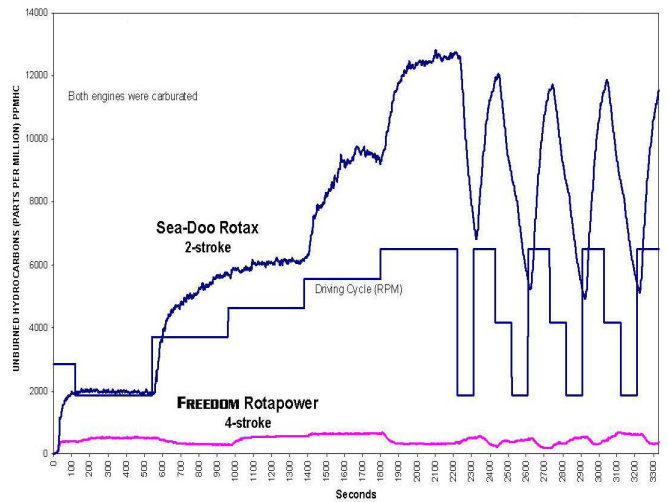
Emission Comparison CARB El Monte Test Facility (12/2/98) 1998 SEA-DOO Rotax 2-stroke 90 HP vs. Freedom Rotapower 4-stroke 110 HP
